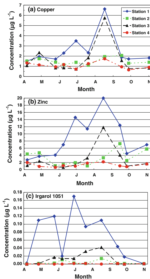
Fig. 1 Concentrations of a copper, b zinc, and c Irgarol 1051 in the Stockholm Archipelago during the boating season April–November 2004. Station 1 Bullandö Marina, Station 2 sound outside the marina, Station 3 natural harbour at Säck, Station 4 Fjärdgrundet
